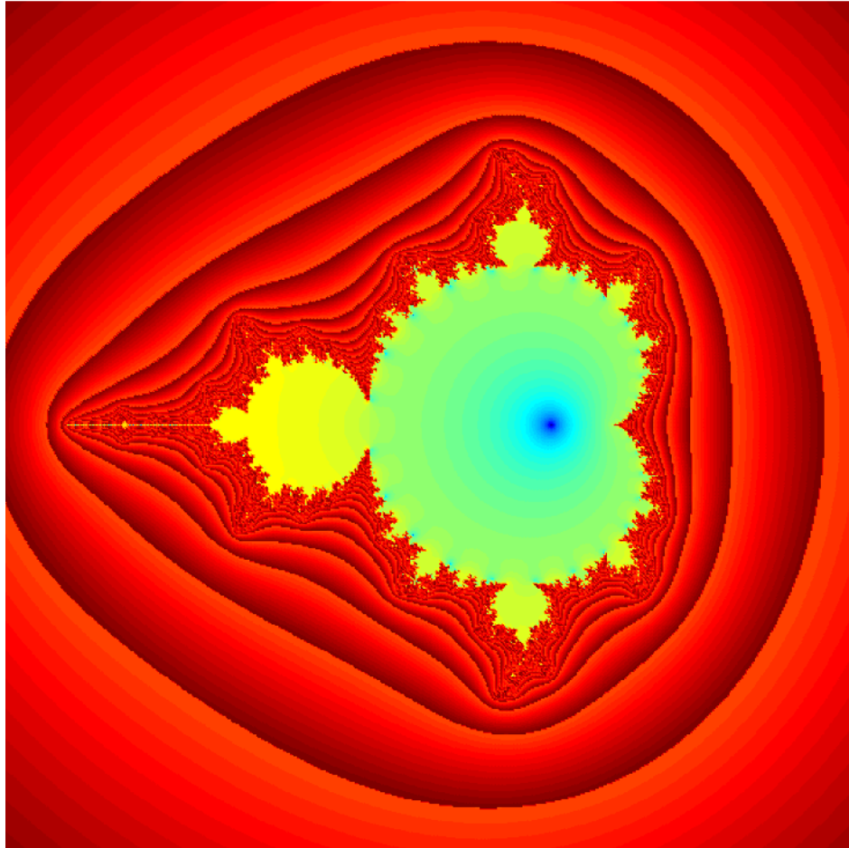
Mandelbrot set, 501 x 501 pixels, 30 iterations
